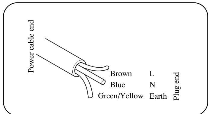
Connection diagram of the AC power cable for 200 V to 240 V
